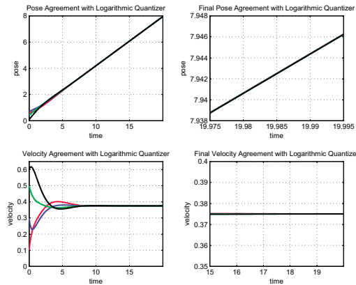
Fig. 6. Second order system with logarithmic quantizers.
